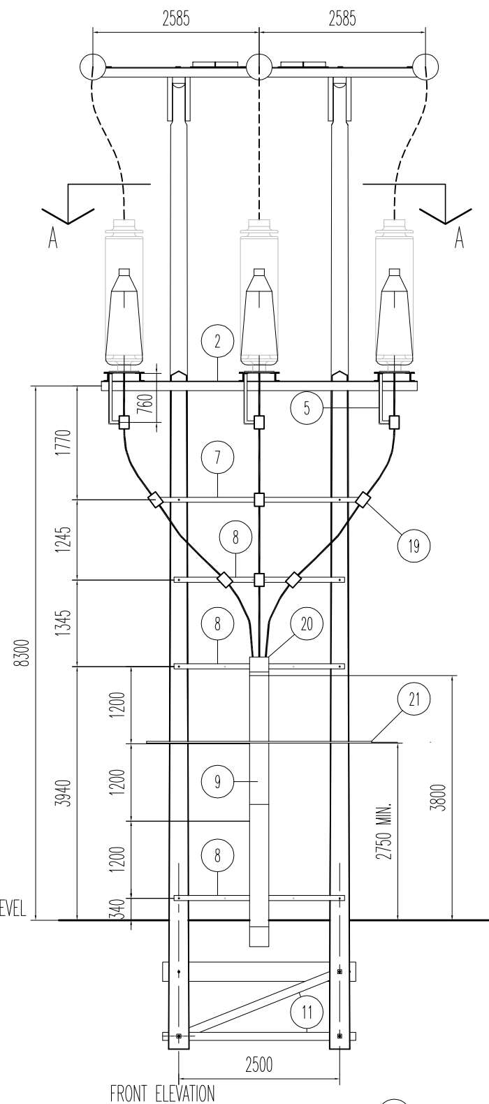
PART DETAIL OF FRONT ELEVATION
