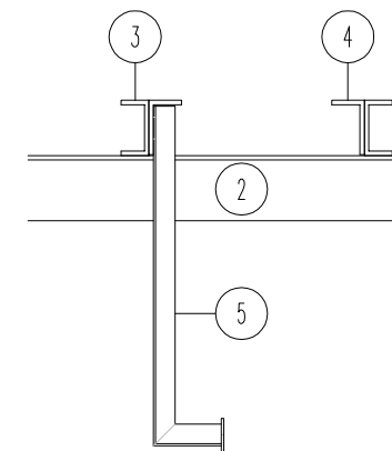
PART DETAIL OF FRONT ELEVATION
